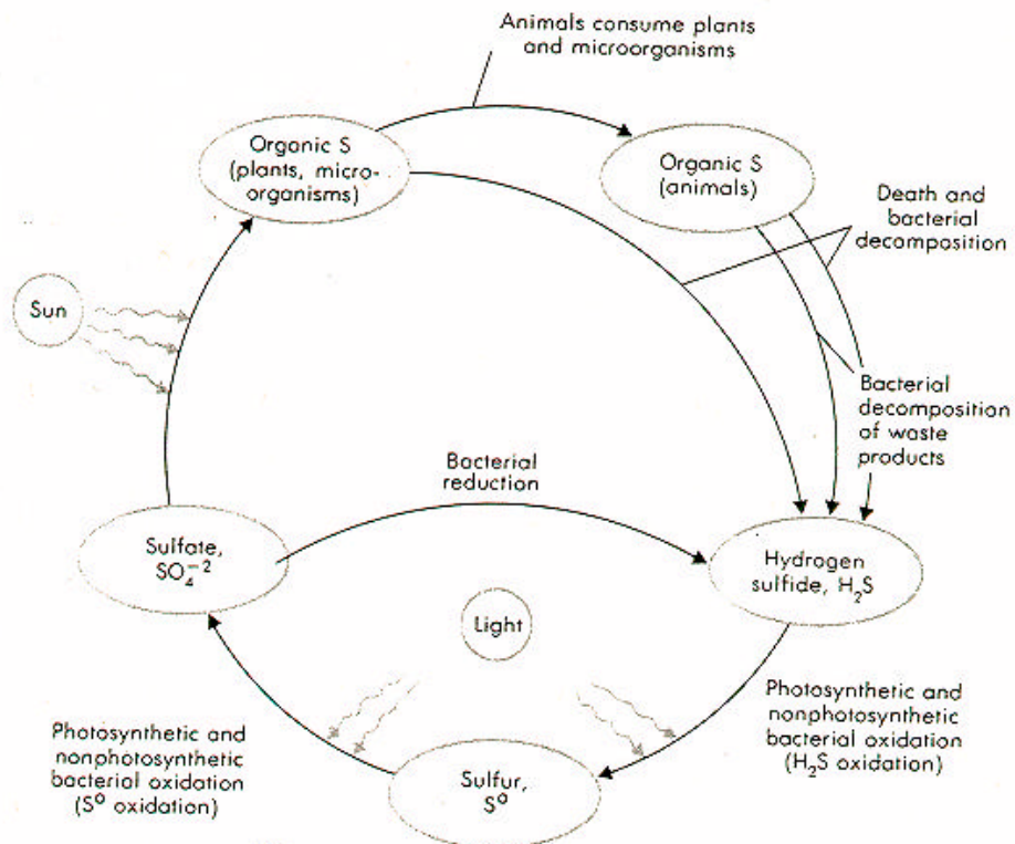
Simplified Sulfur Cycle in nature
