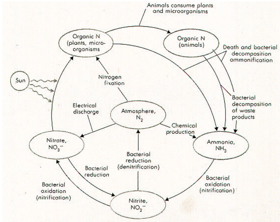
Simplified Nitrogen Cycle in nature
